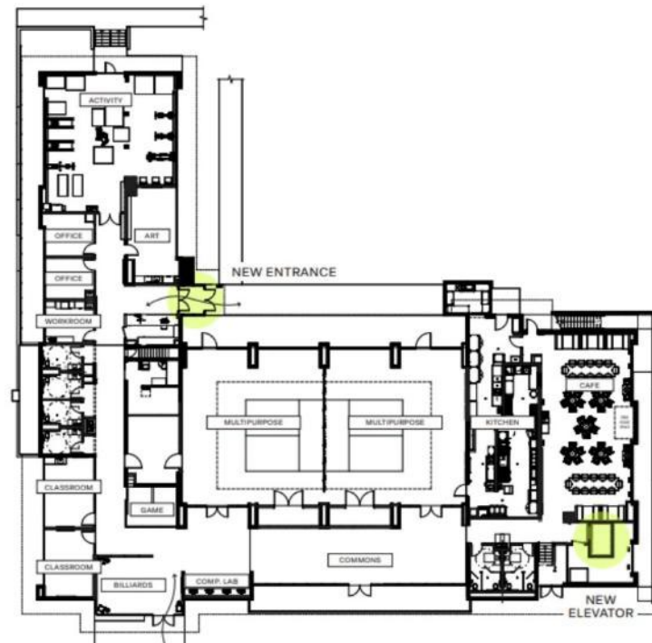
Figure 7 Tenth East Senior Center Renovation Main Level Floor Plan | Nexus Architecture
