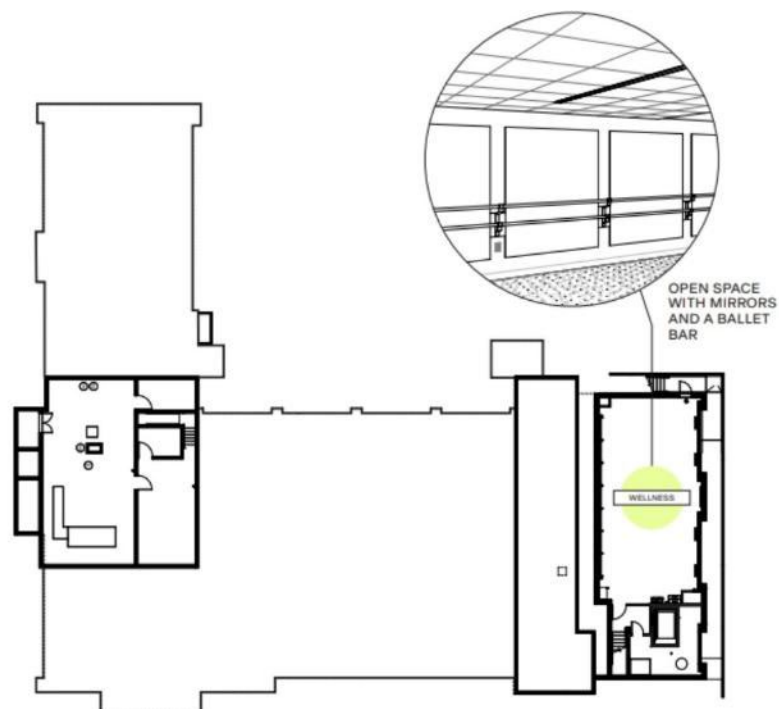
Figure 8 Tenth East Senior Center Renovation Lower Level Floor Plan | Nexus Architecture
